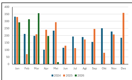
Figure 5 Monthly Rainfall Graph (2024–2026) at the Catchment Area of Void Melawan Panel 2
