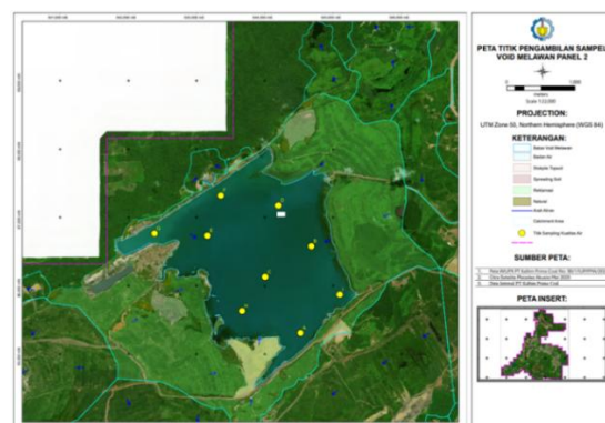
Figure 1 Location Map and Water Quality Sampling Points of Void Melawan Panel 2
