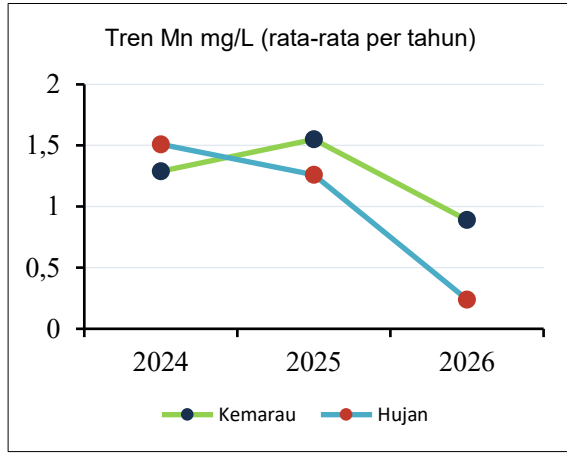
Figure 9 Annual Mean Mn Trend at Void Melawan Panel 2
