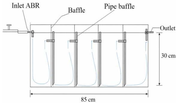
Figure 1. Anaerobic Baffle Reactor Design
