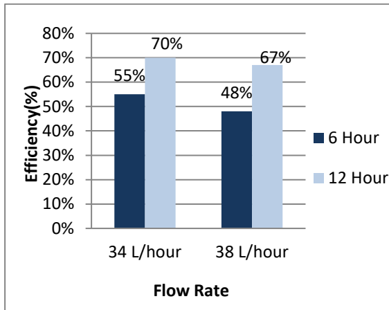
Figure 2. Ammonia Reduction Efficiency
