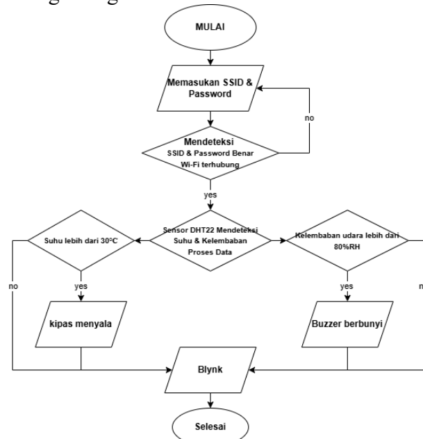
Gambar 3. Flowchart
